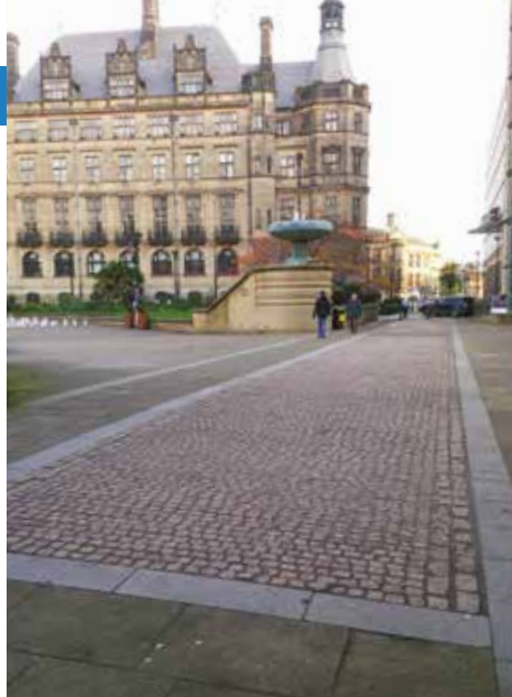
⤴ ProJoint™ V400-WT (black) in Sheffield City Centre
